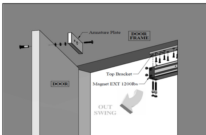
Explode View
