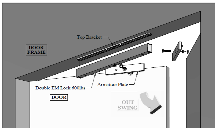
Explode View
