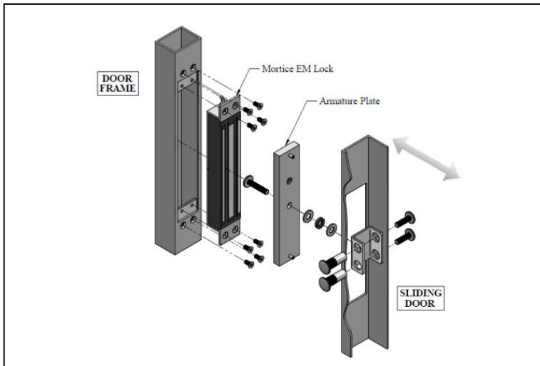
Explode View
