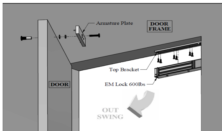
Explode View
